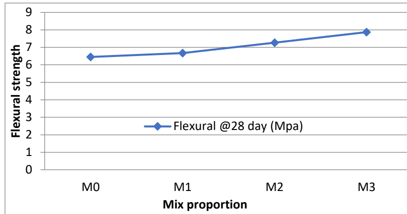
The figure for flexural strength at 28days
